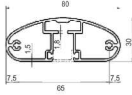
* 7800 Elips Cam Profili 1,221 kg/mt
